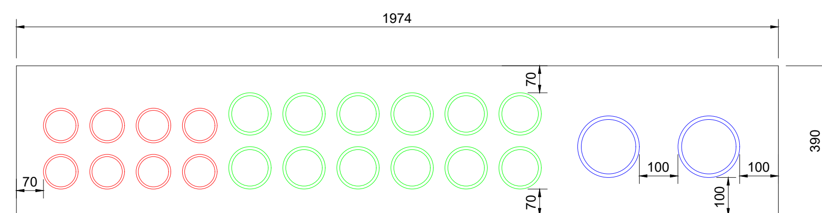
STM-08B ESC. 1/10
