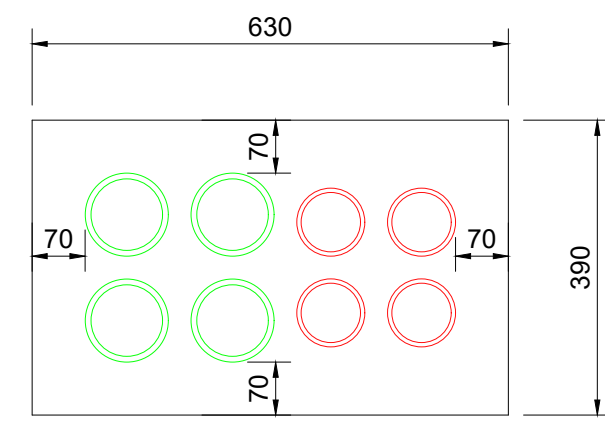
STM-06B ESC. 1/10
