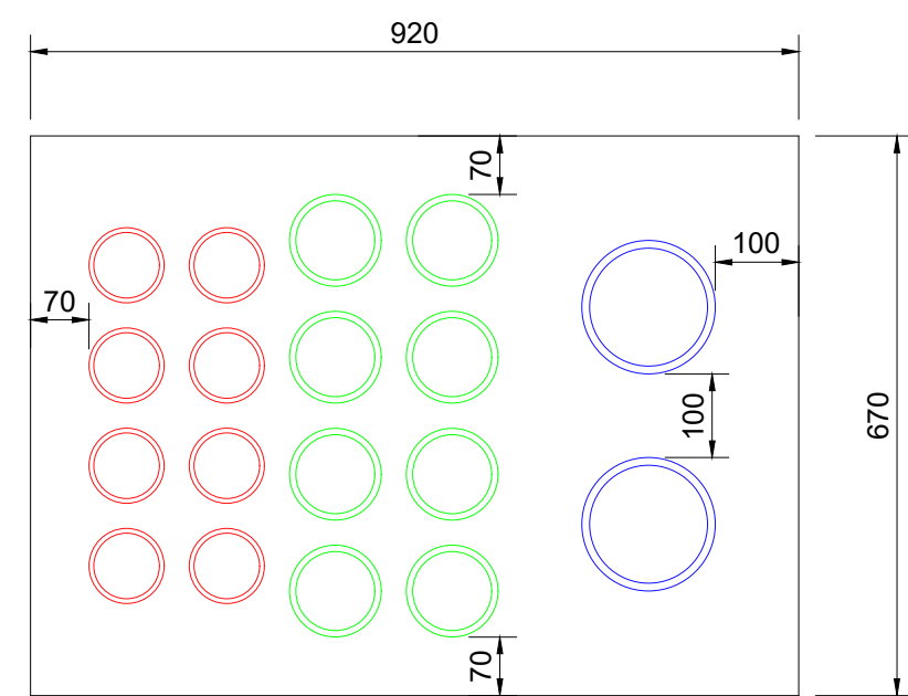
STM-01B ESC. 1/10
